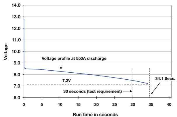
Figure 5: CCA test @ -40°C on 31-PC2150
