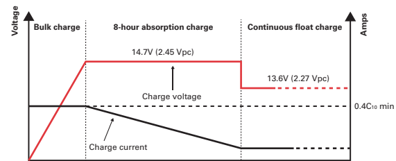
Figure 6: Recommended three-step charge profile
